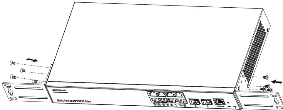
Install on 19" Standard Rack
