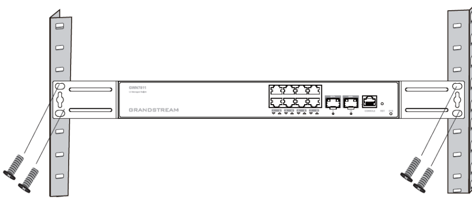
Install on 19" Standard Rack
