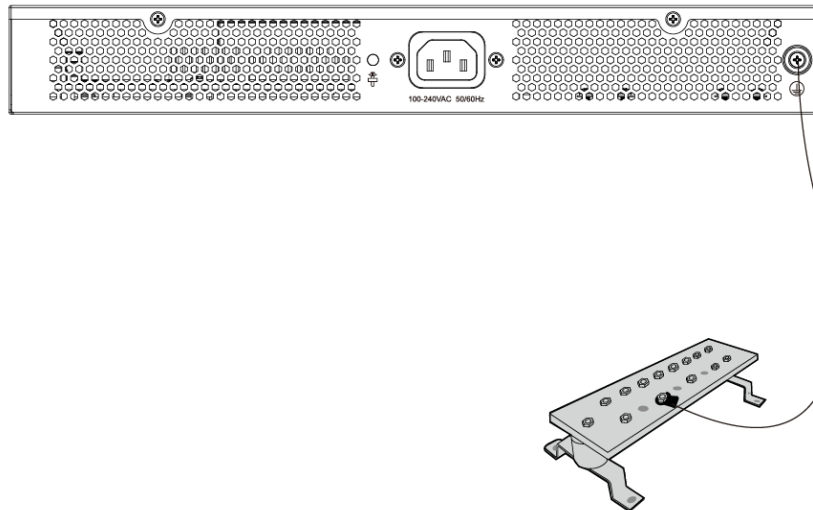
Grounding the Switch
